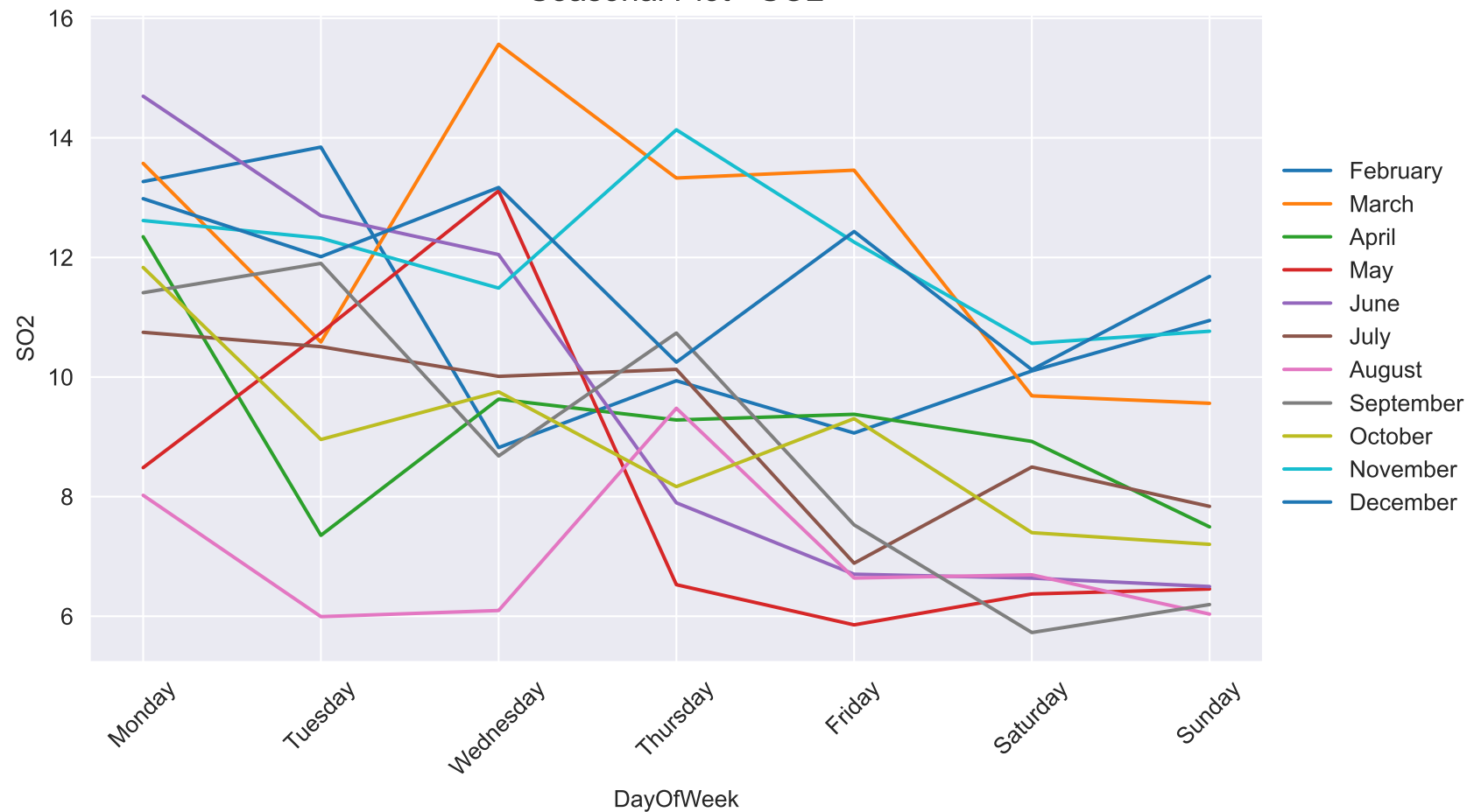
Seasonal Plot - SO2
