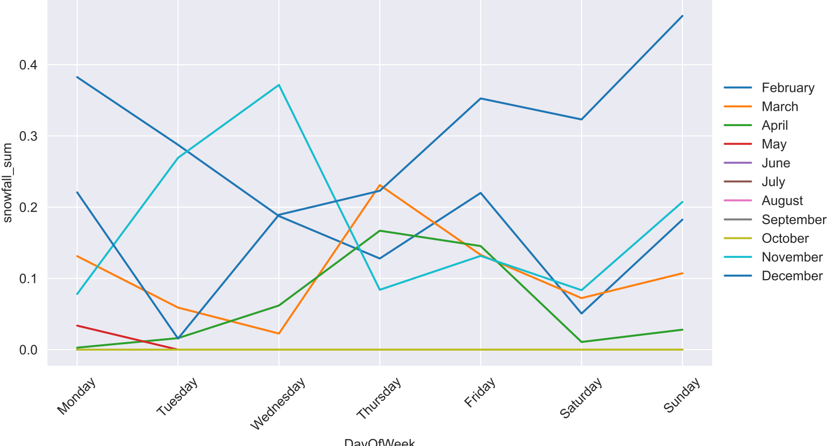
Seasonal Plot - snowfall sum
