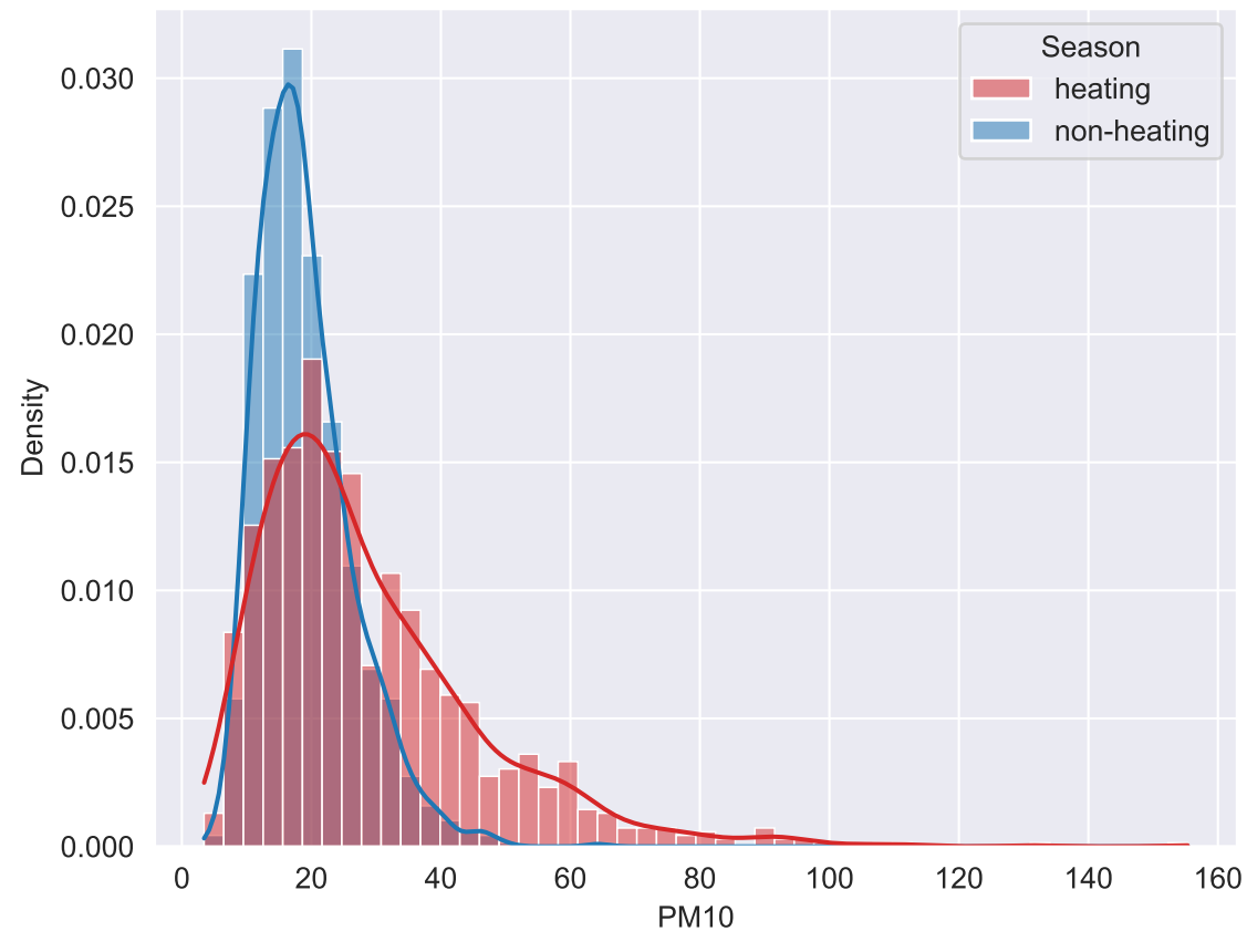
Histogram grouped by seasons and working days - PM10
