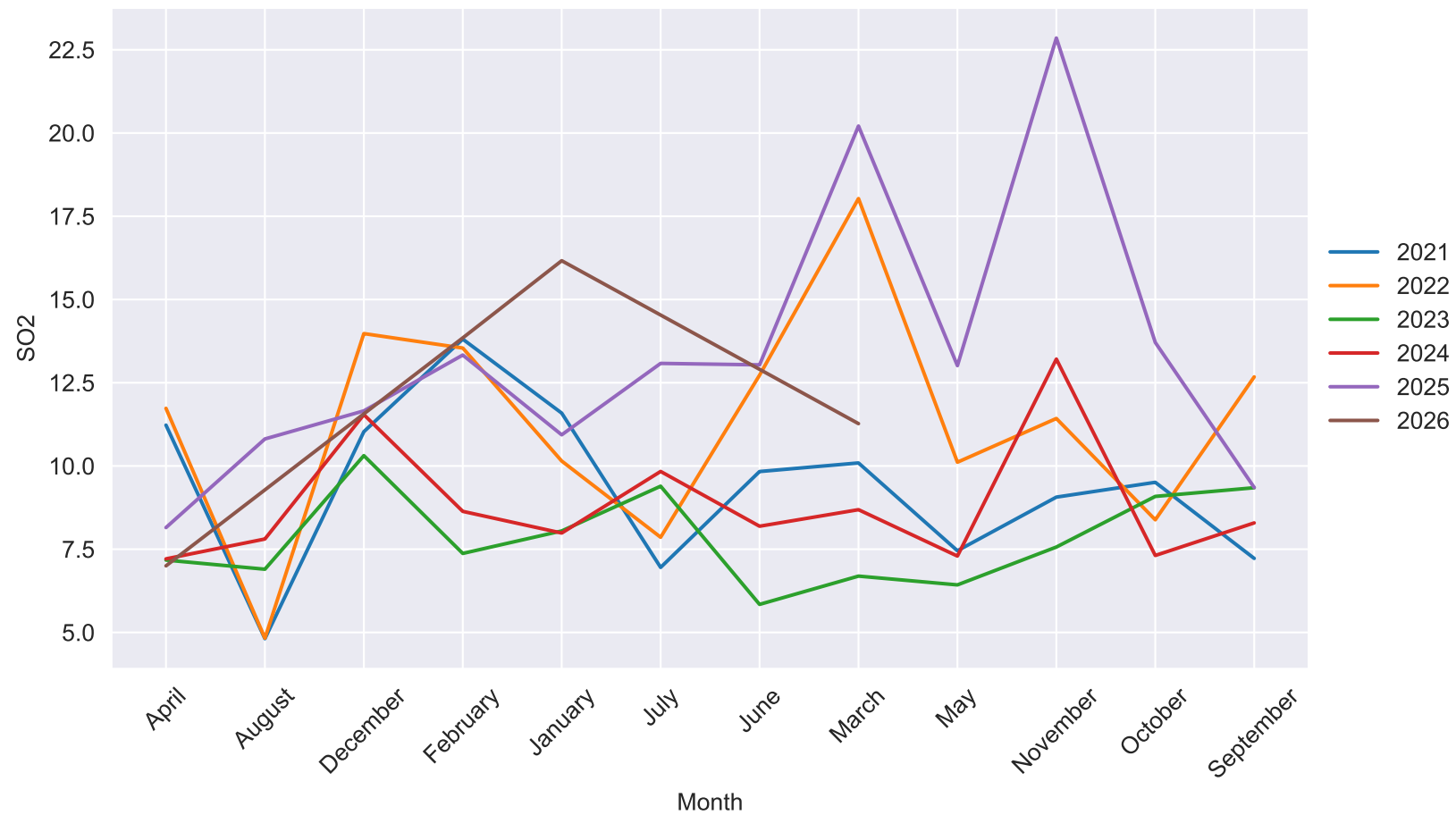
Seasonal Plot - SO2
