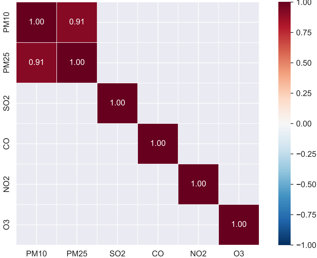
Spearman correlation of pollutants where |r_s| \geq 0.9
