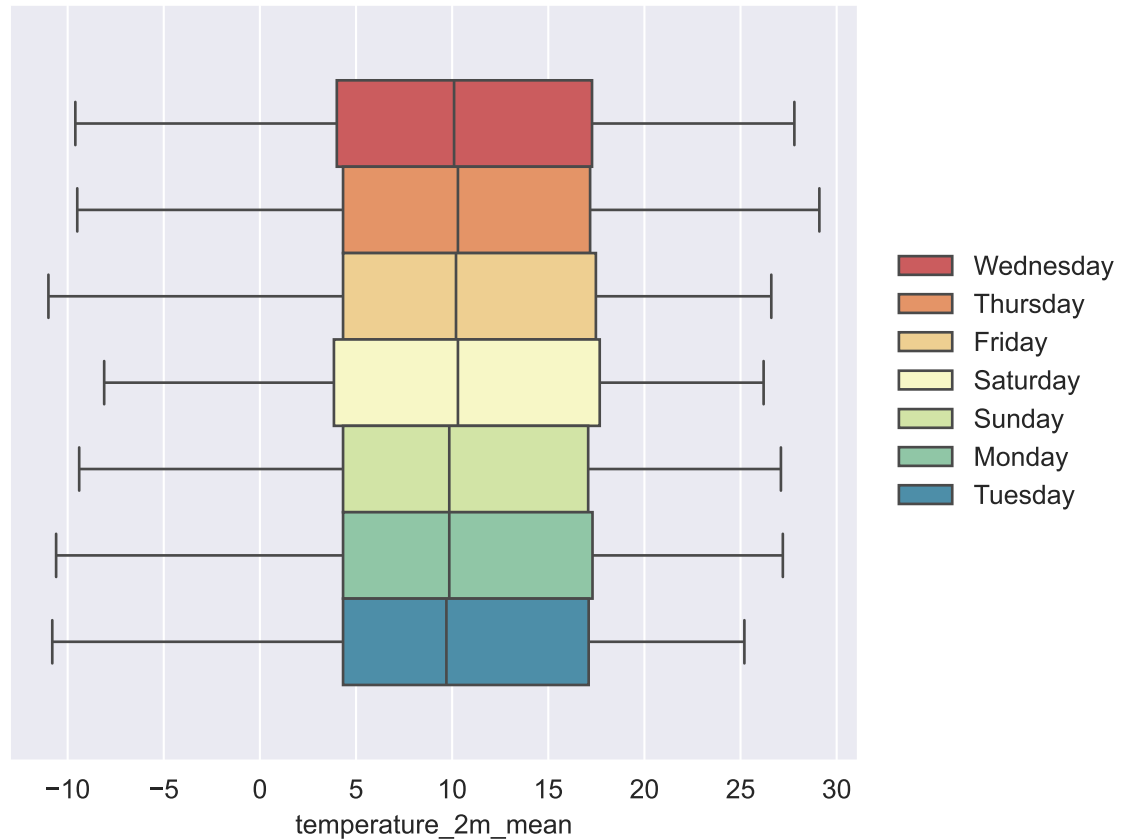
Boxplots of temperature_2m_mean by Month and by Weekday
