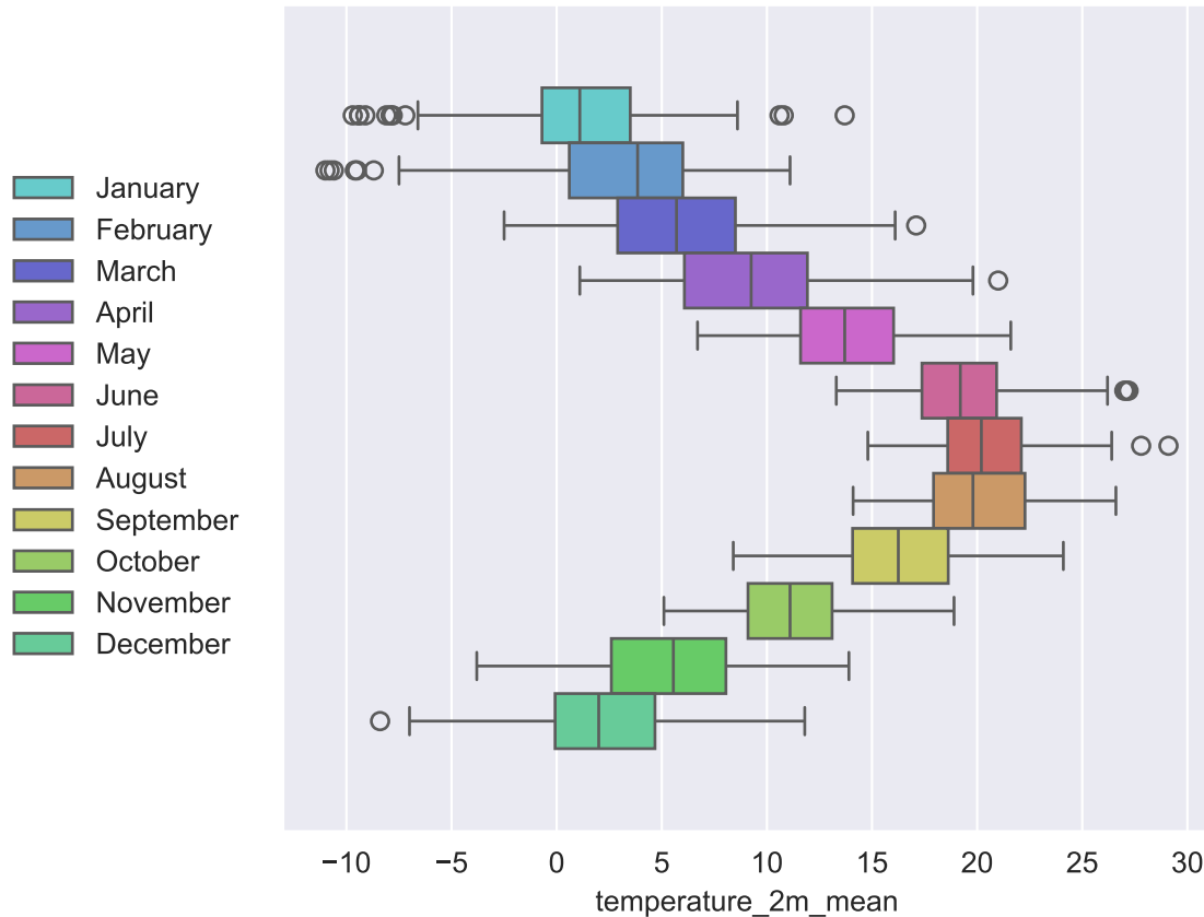
Boxplots of temperature_2m_mean by Month and by Weekday
