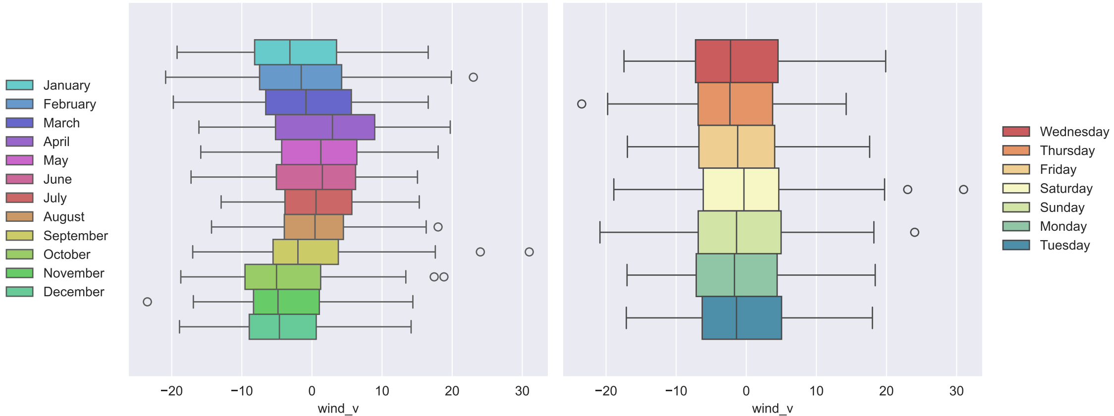
Boxplots of wind_v by Month and by Weekday
