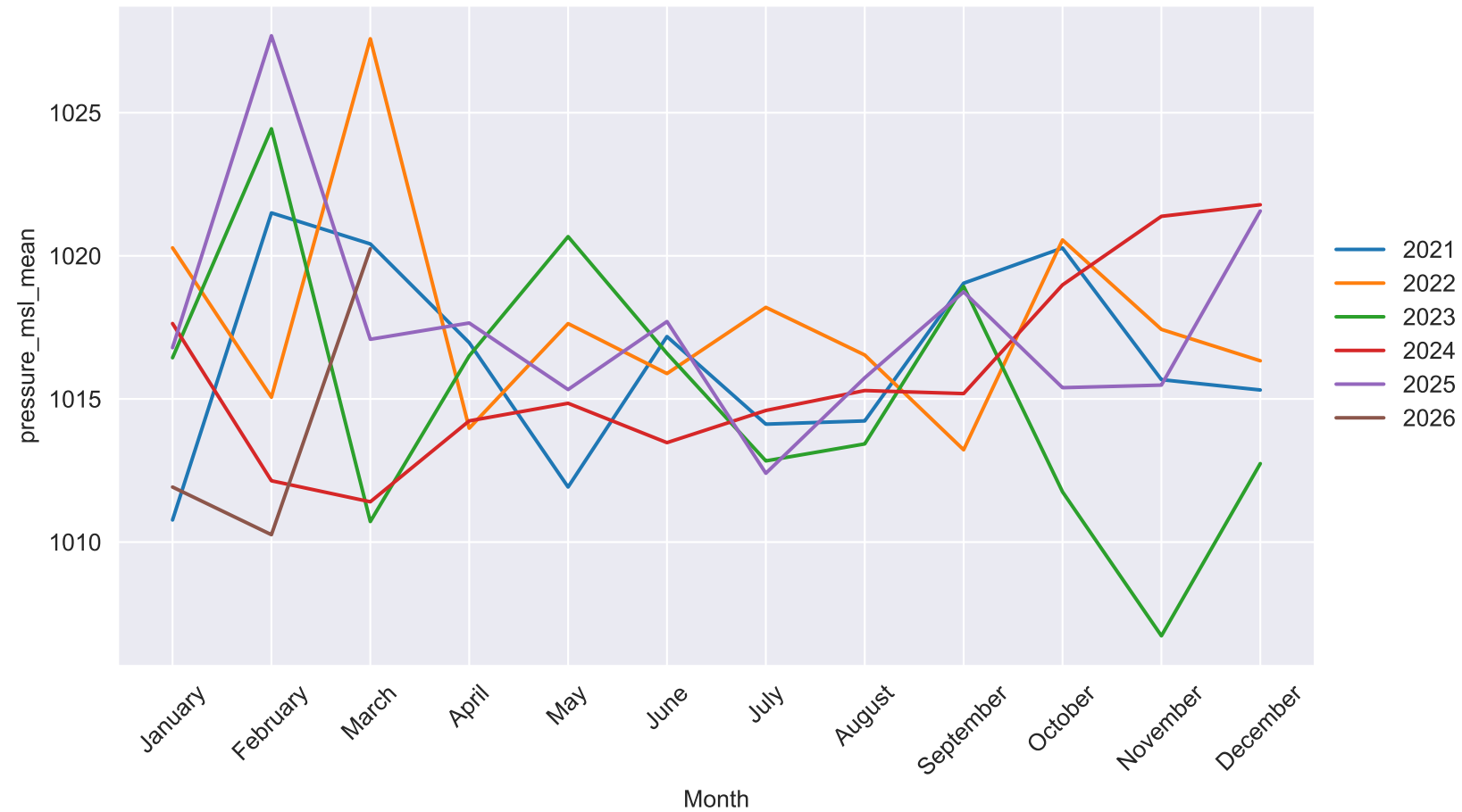
Seasonal Plot - pressure_msl_mean
