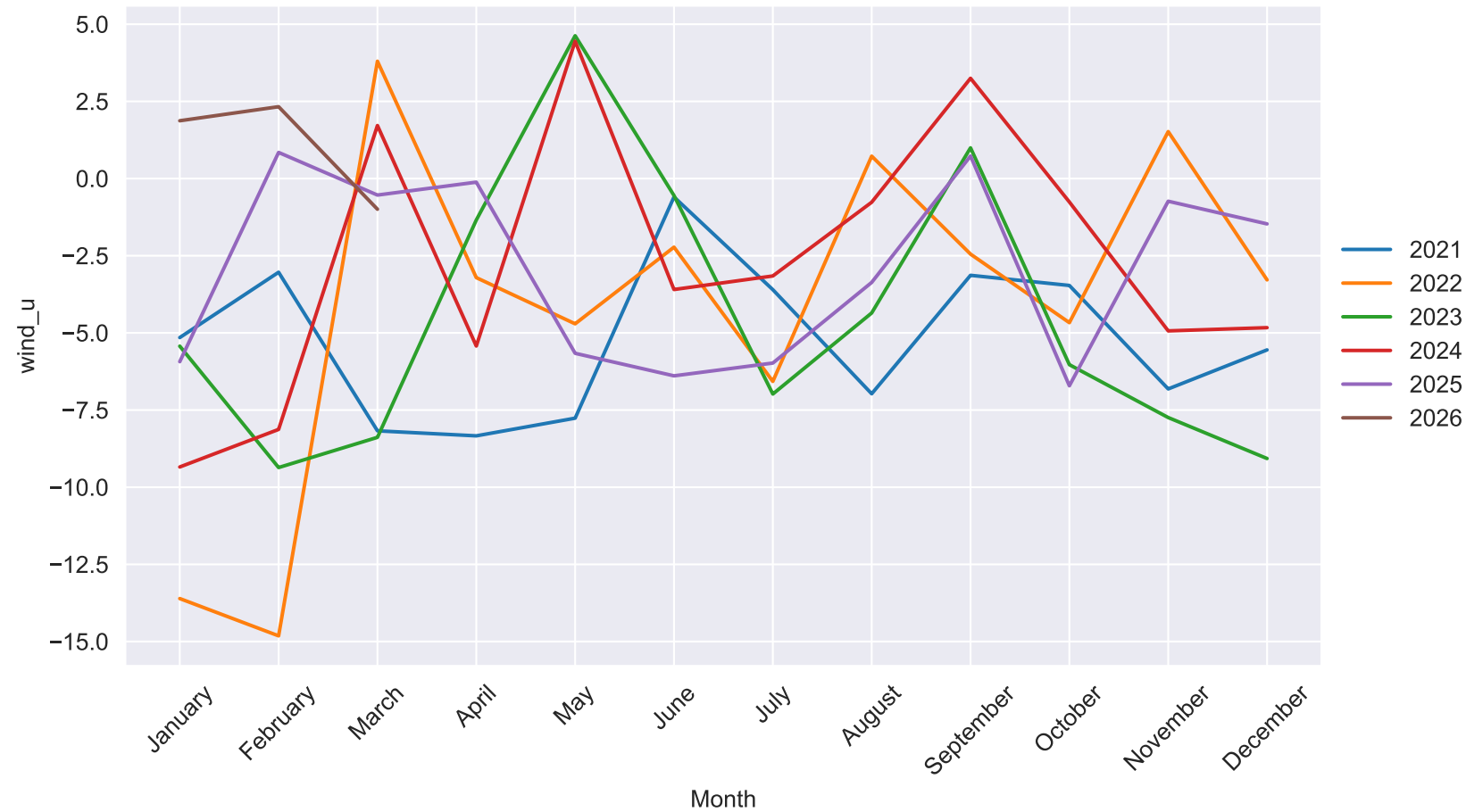
Seasonal Plot - wind_u
