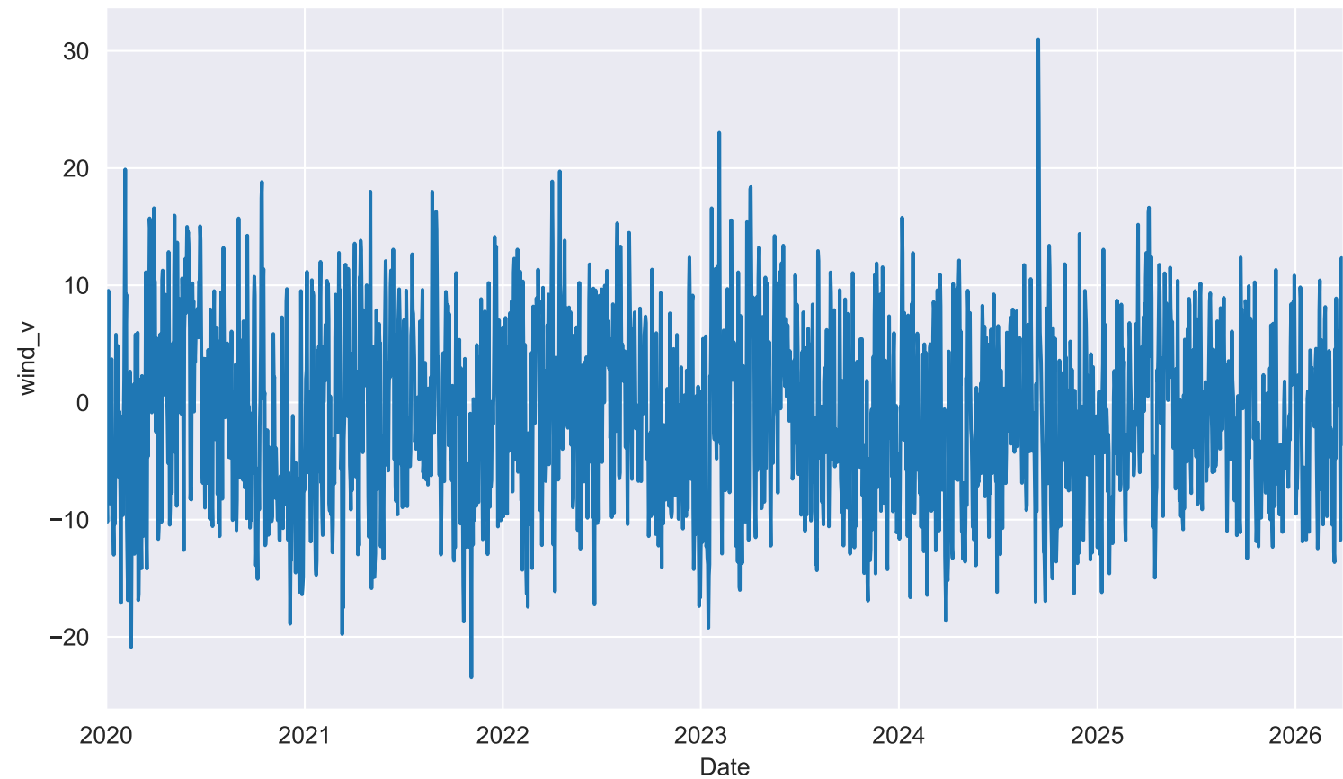
Time series: wind_v
