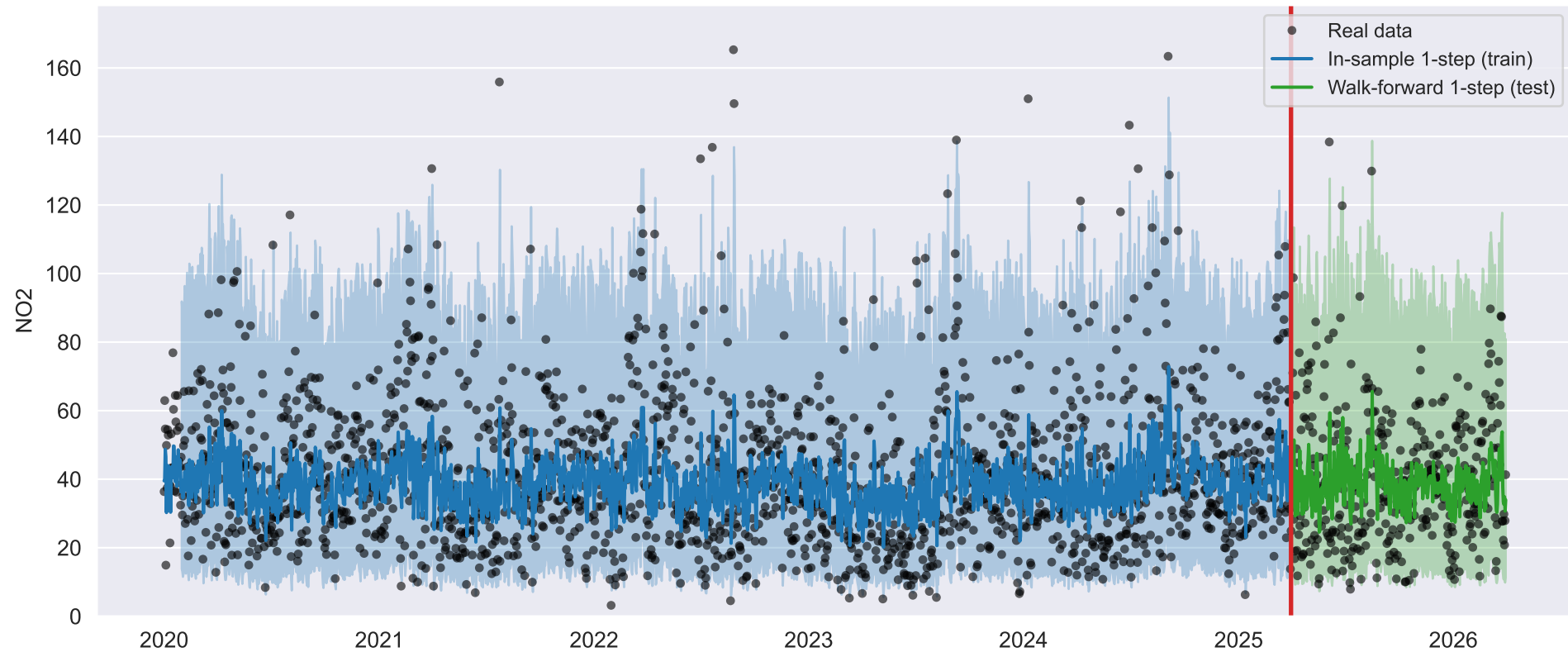
VAR (stationary) — NO2
