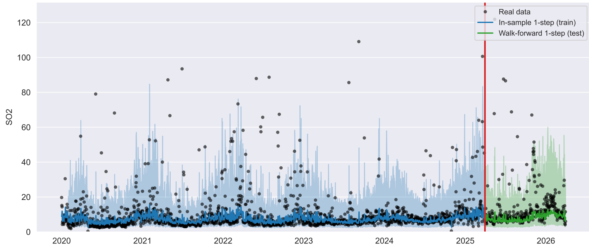
VAR (stationary) — SO2
