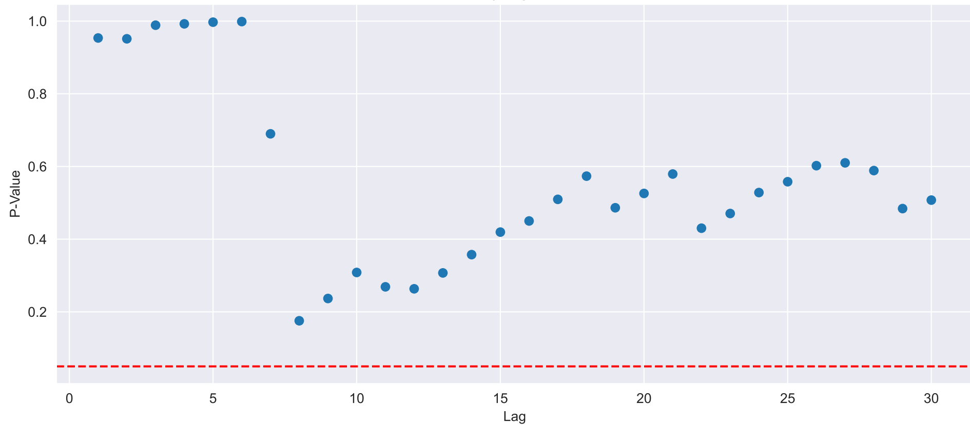
P-value from Ljung-Box test - SO2
