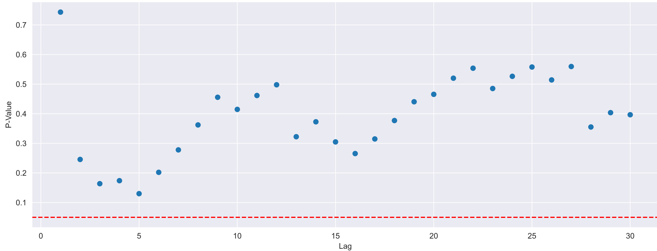
P-value from Ljung-Box test - PM25
