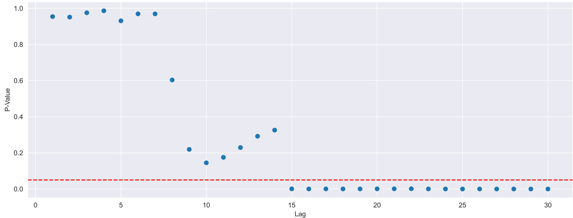
P-value from Ljung-Box test - NO2
