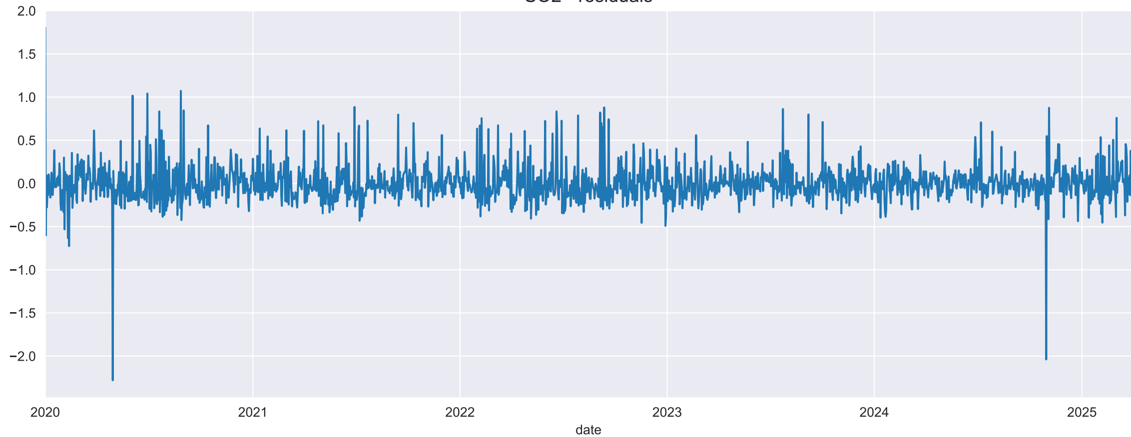
SO2 - residuals
