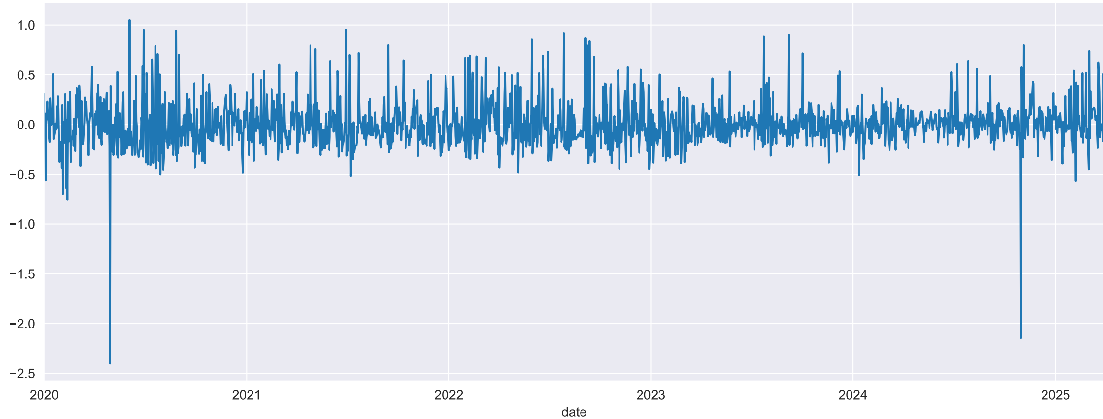
SO2 - residuals
