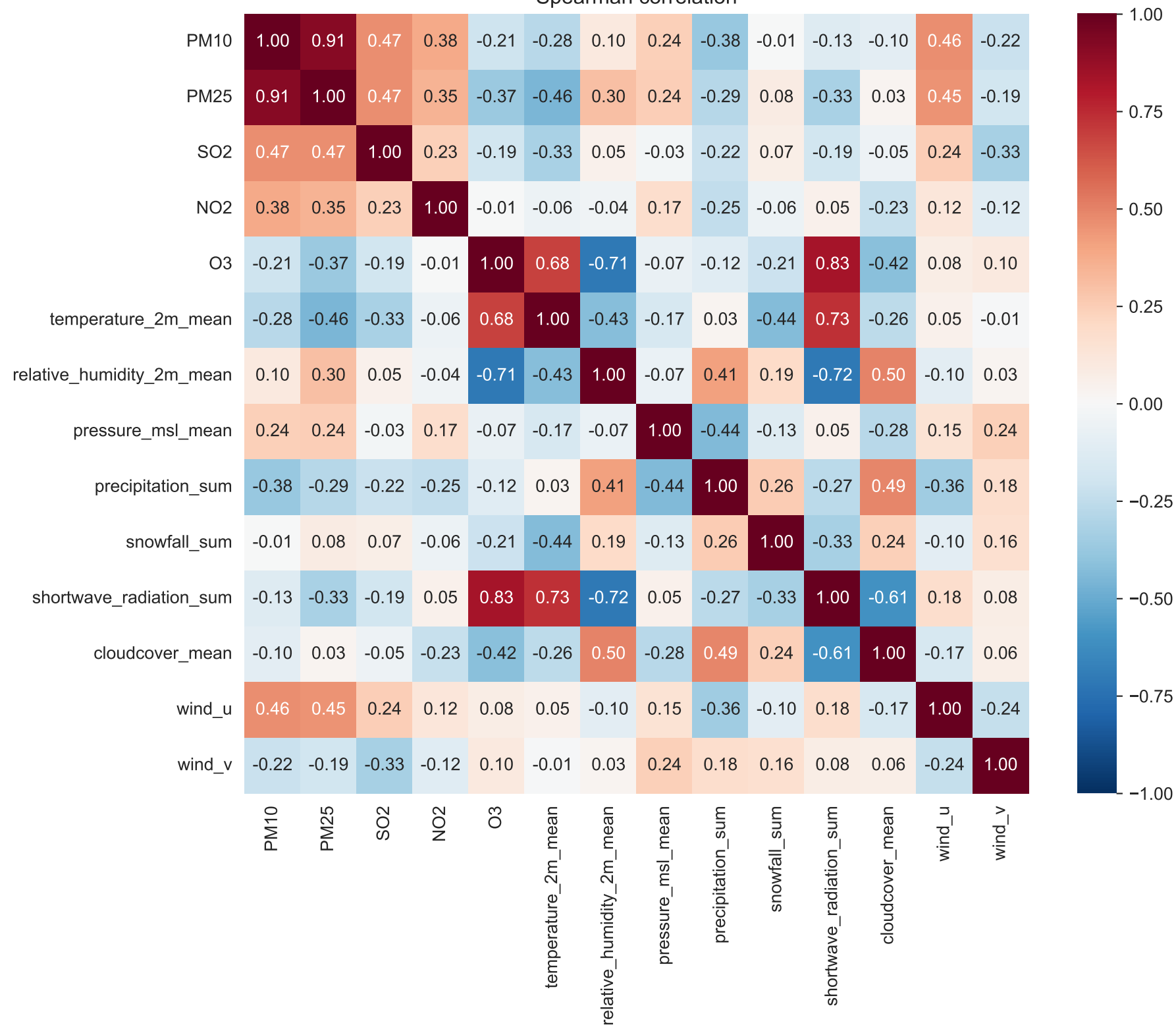
Spearman correlation
