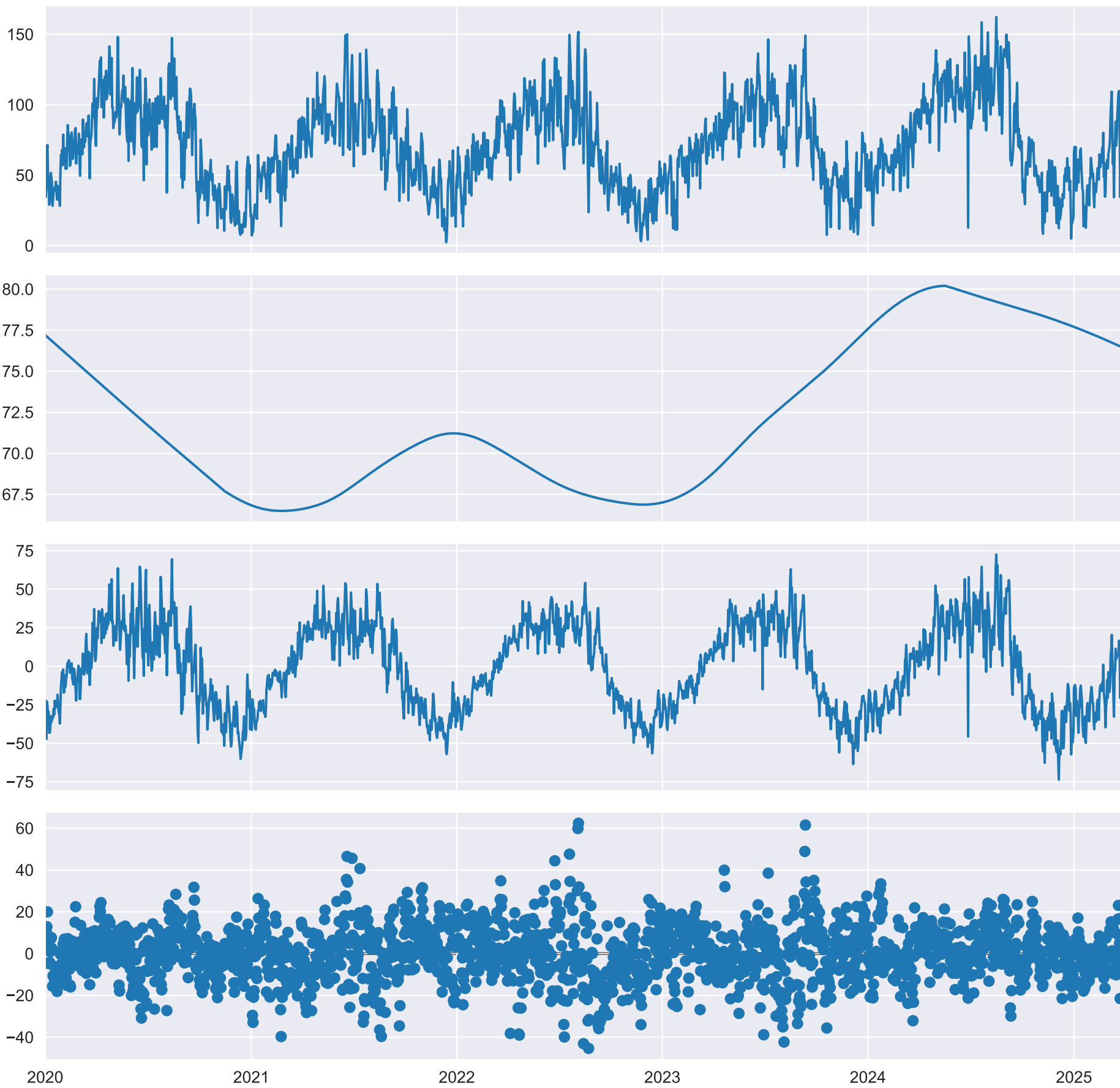
STL Decomposition of O3
