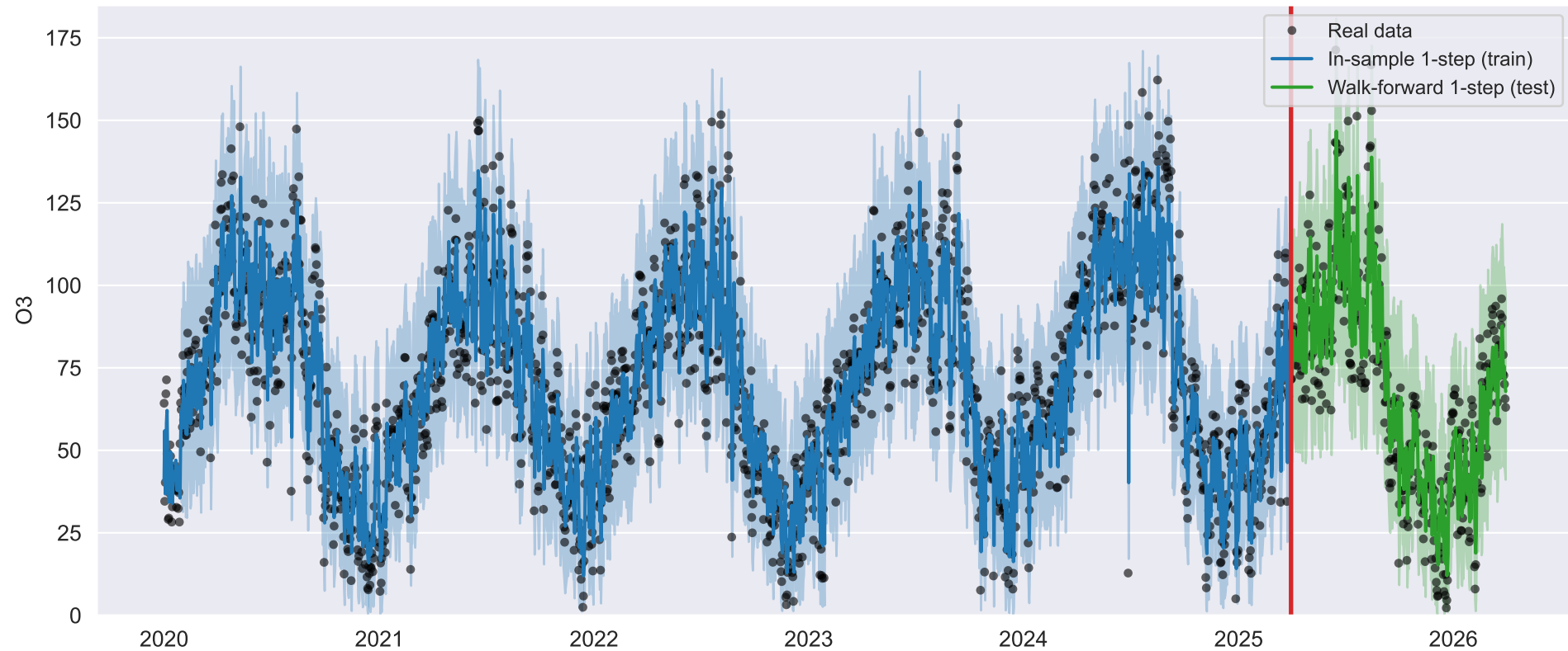
VAR (stationary) — O3
