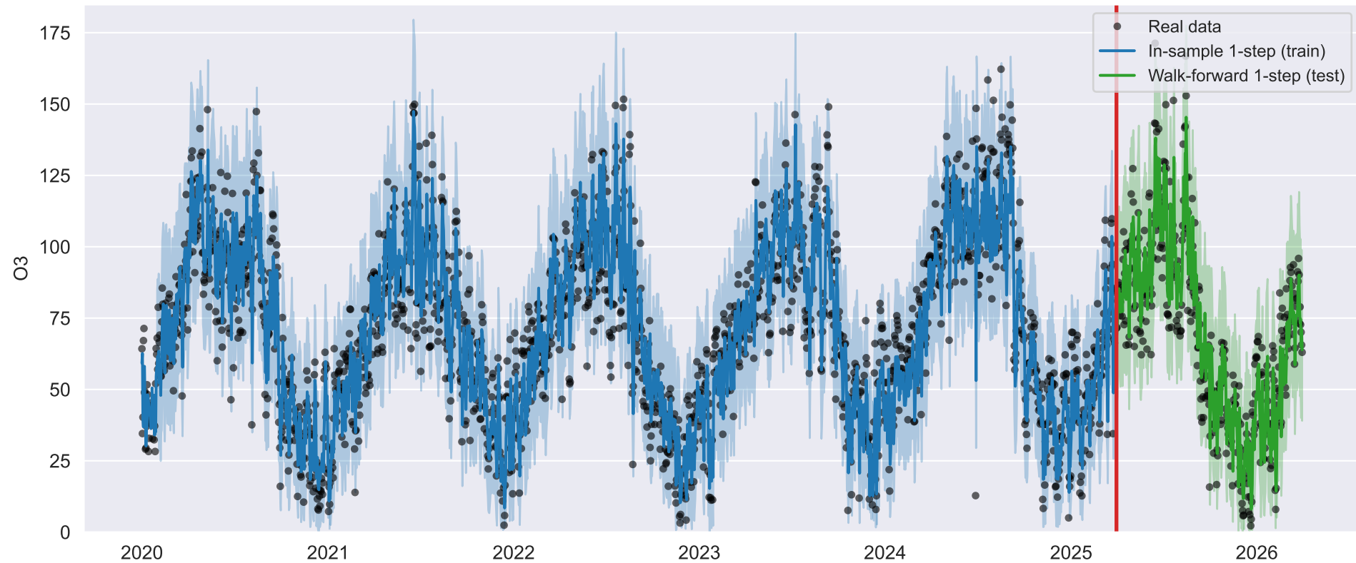
VAR (stationary + meteo) — O3
