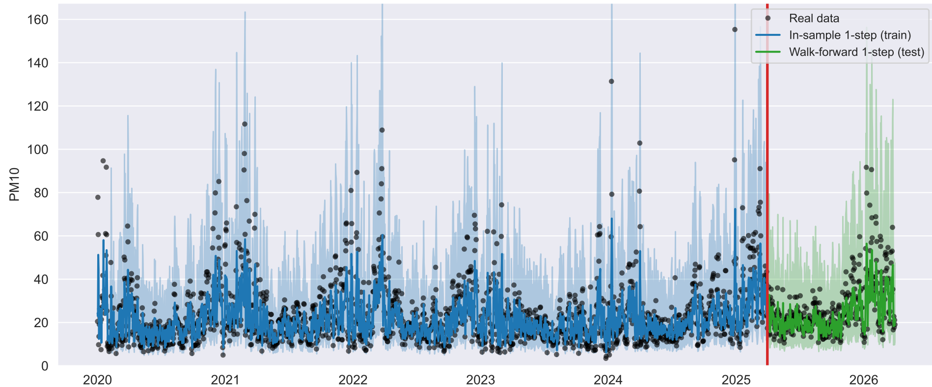
VAR (stationary) — PM10
