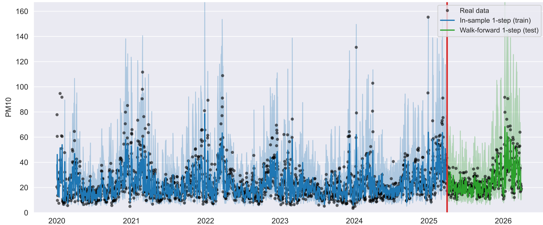
VAR (stationary + meteo) — PM10
