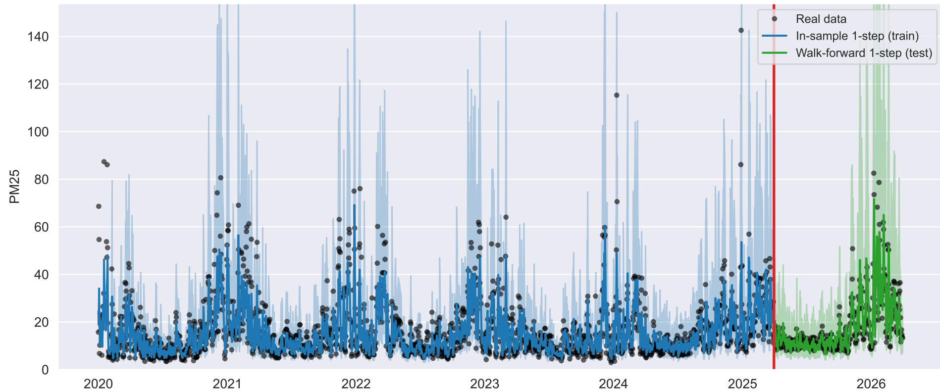
VAR (stationary + meteo) — PM25
