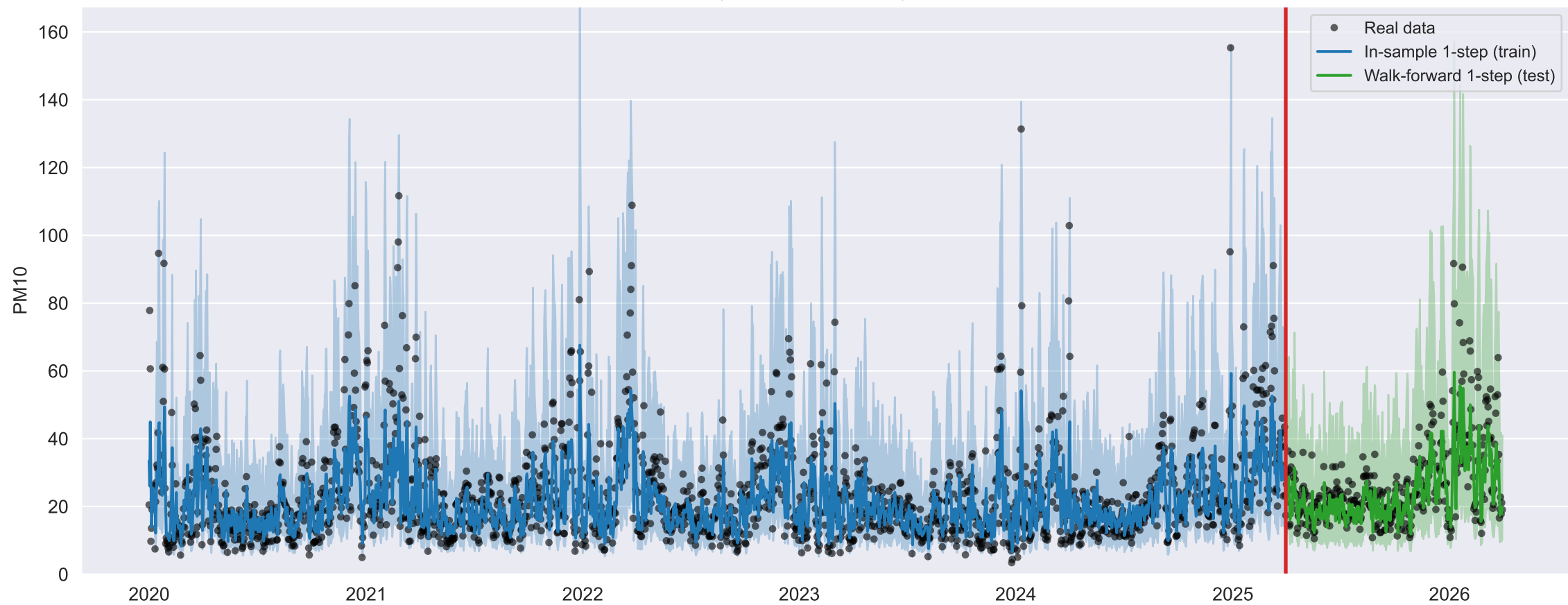
VARX (dummies + meteo) — PM10
