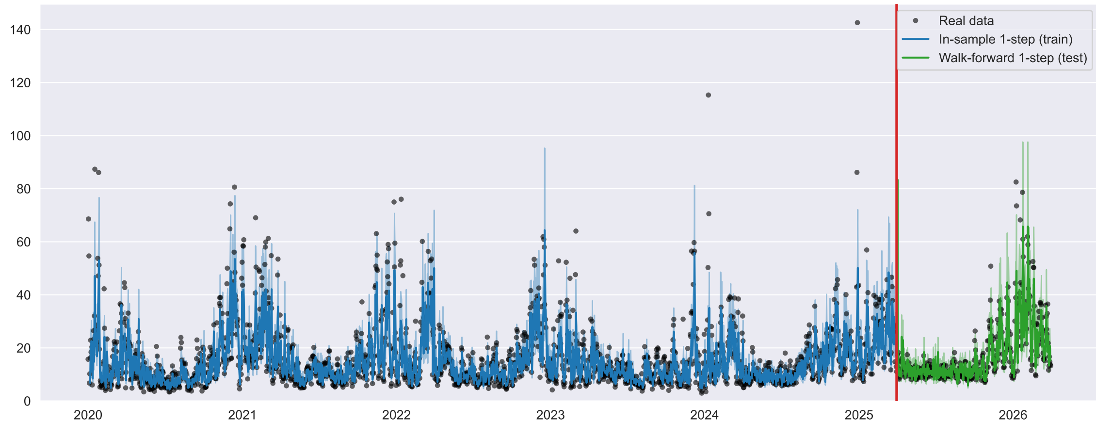
PM25 — in-sample (train) + walk-forward (test)
