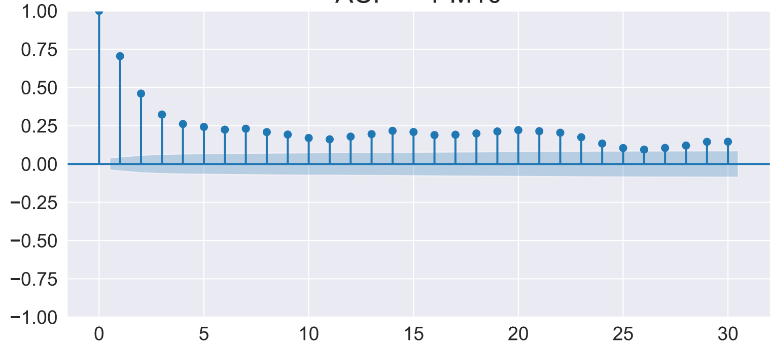
ACF — PM10
