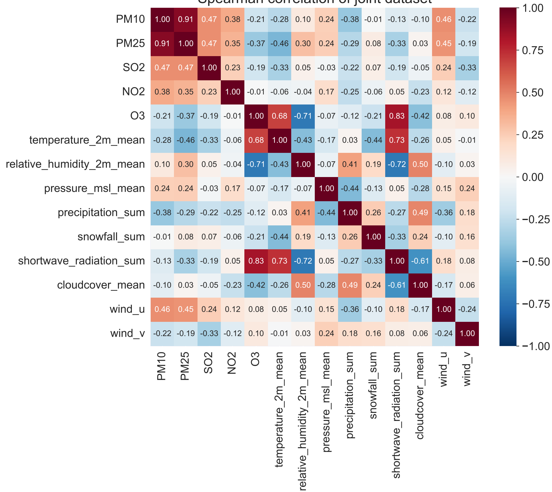
Spearman correlation of joint dataset
