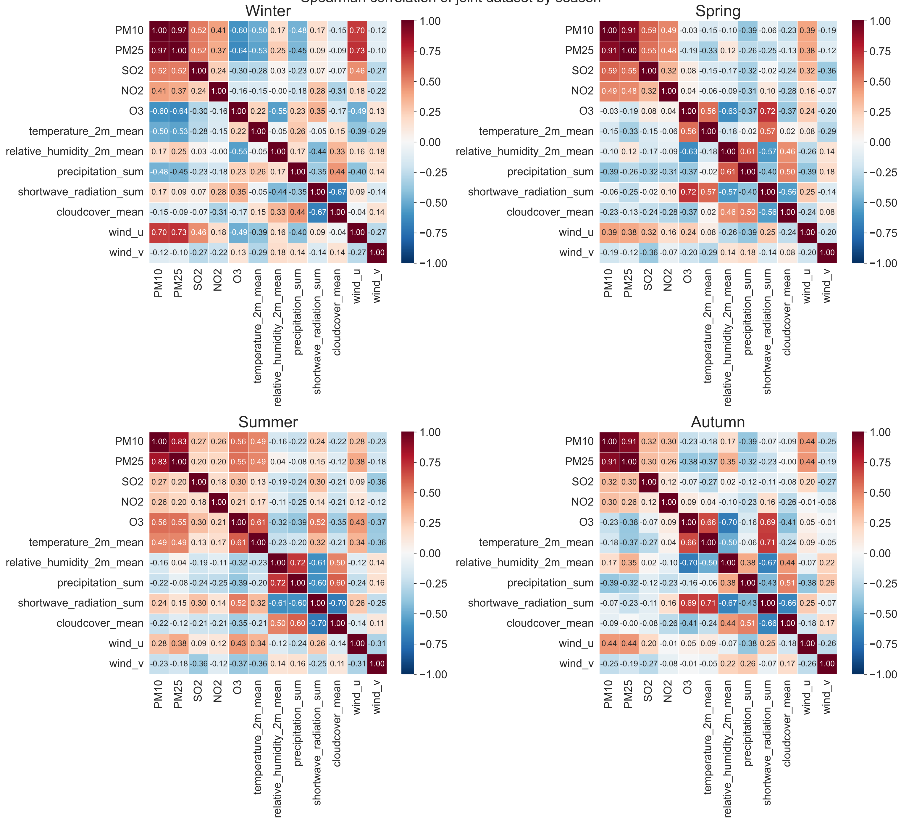
Spearman correlation of joint dataset by season
