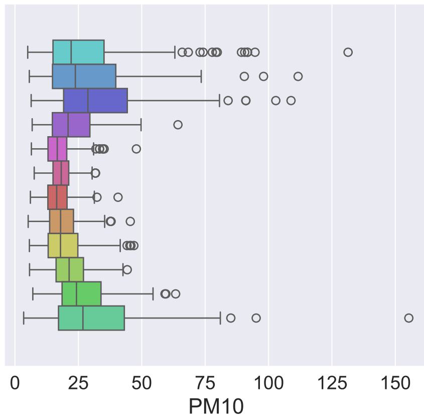
Boxplots of PM10 by Month and by Weekday
