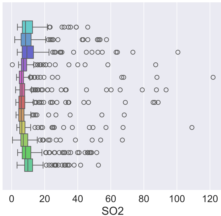
Boxplots of SO2 by Month and by Weekday
