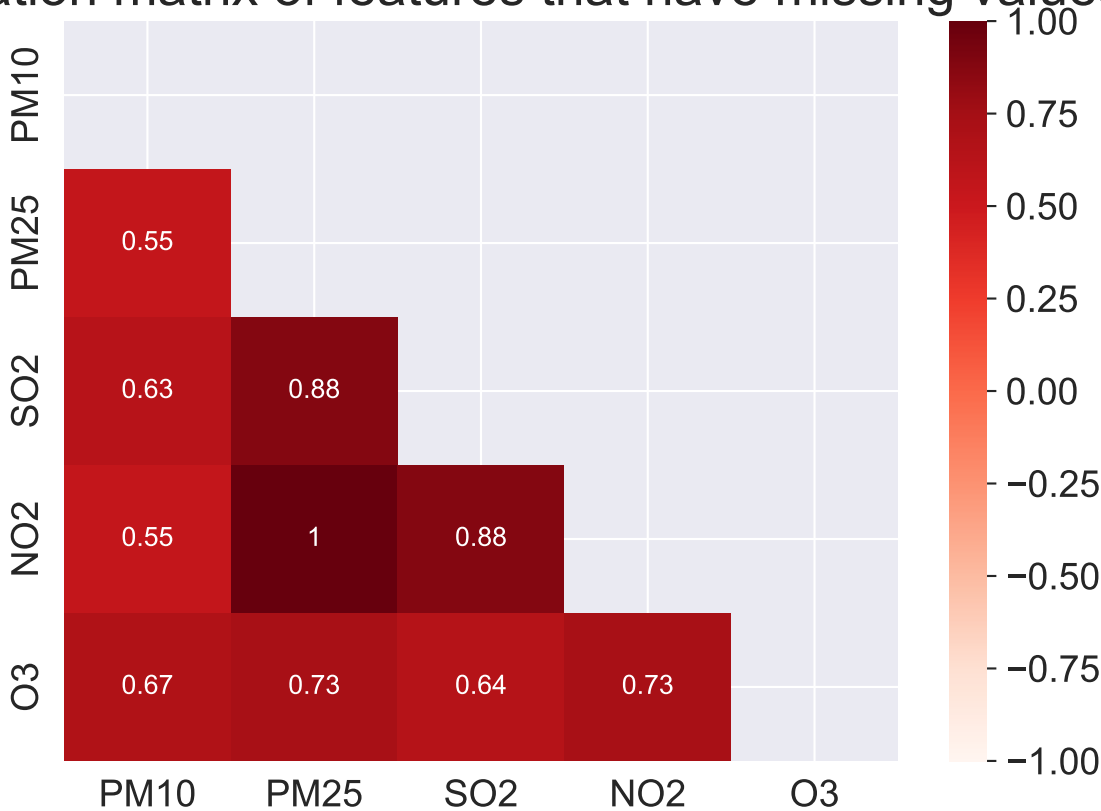
Correlation matrix of features that have missing values
