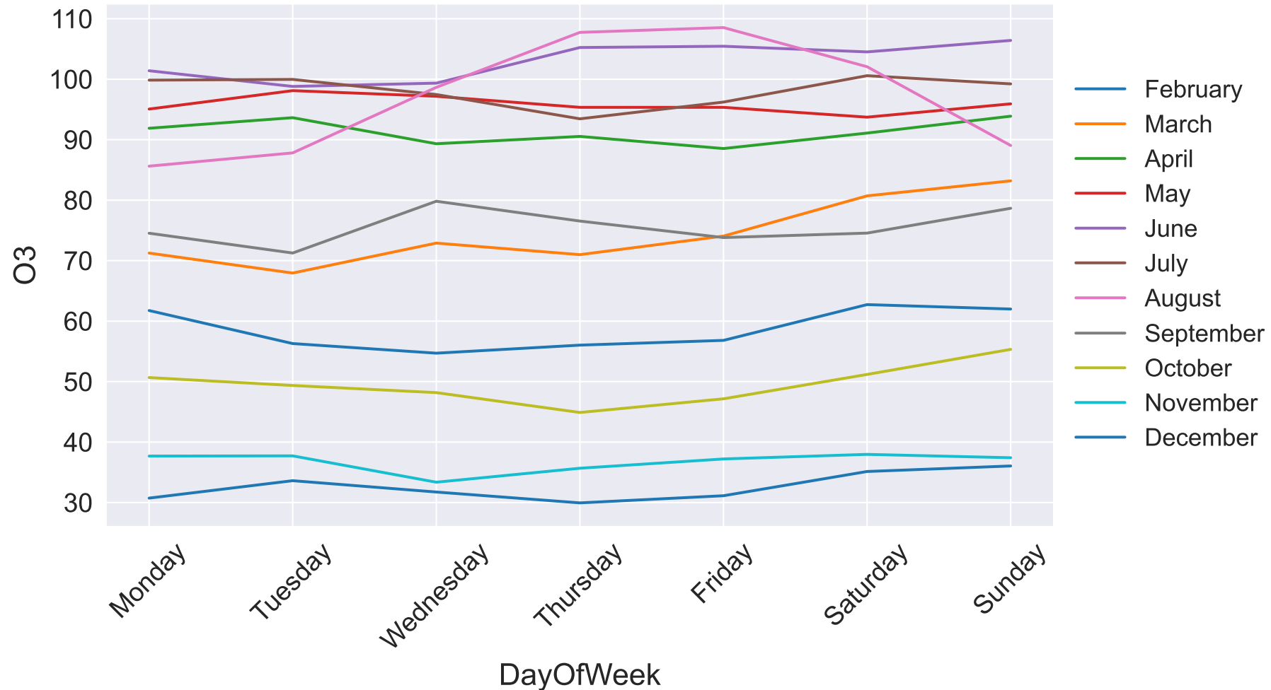
Seasonal Plot - O3
