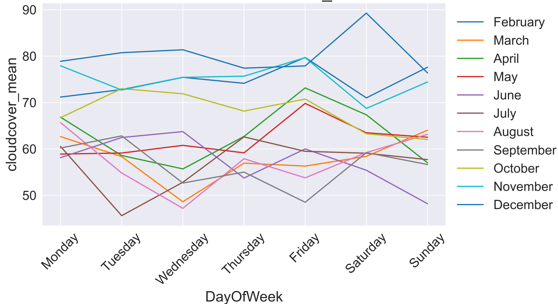
Seasonal Plot - cloudcover_mean
