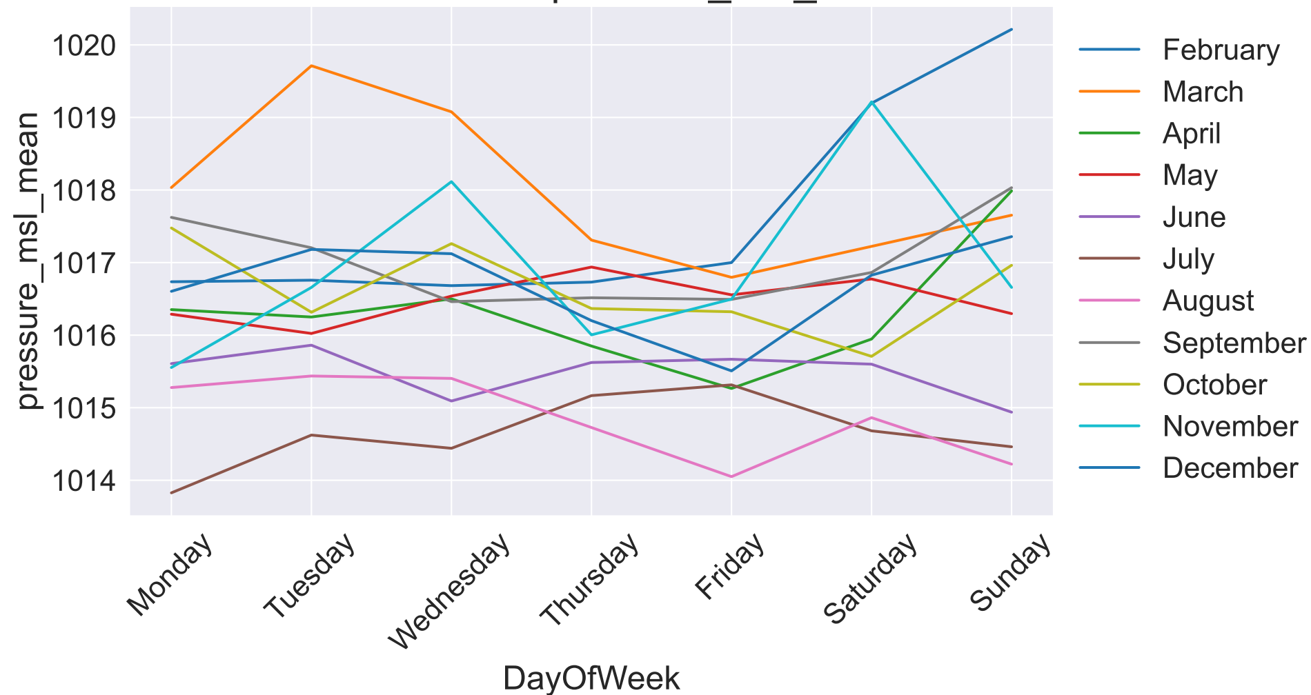
Seasonal Plot - pressure_msl_mean
