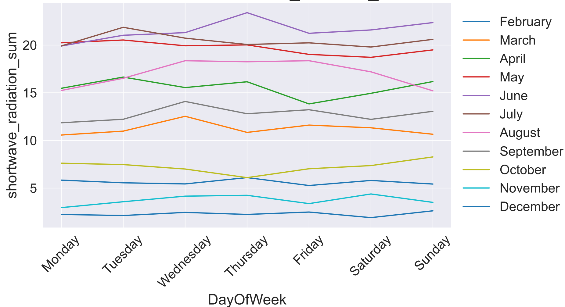
Seasonal Plot - shortwave_radiation_sum
