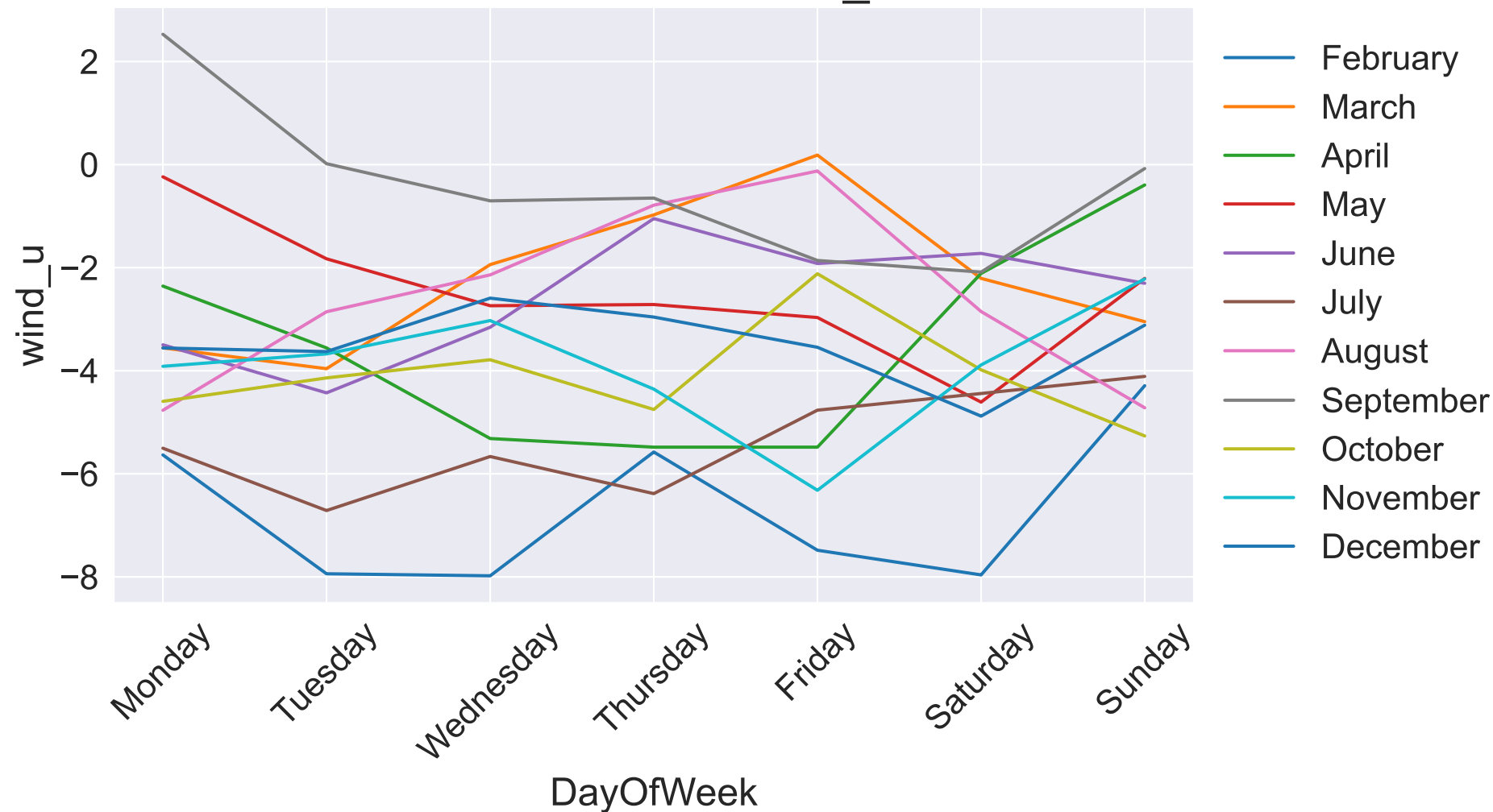
Seasonal Plot - wind_u
