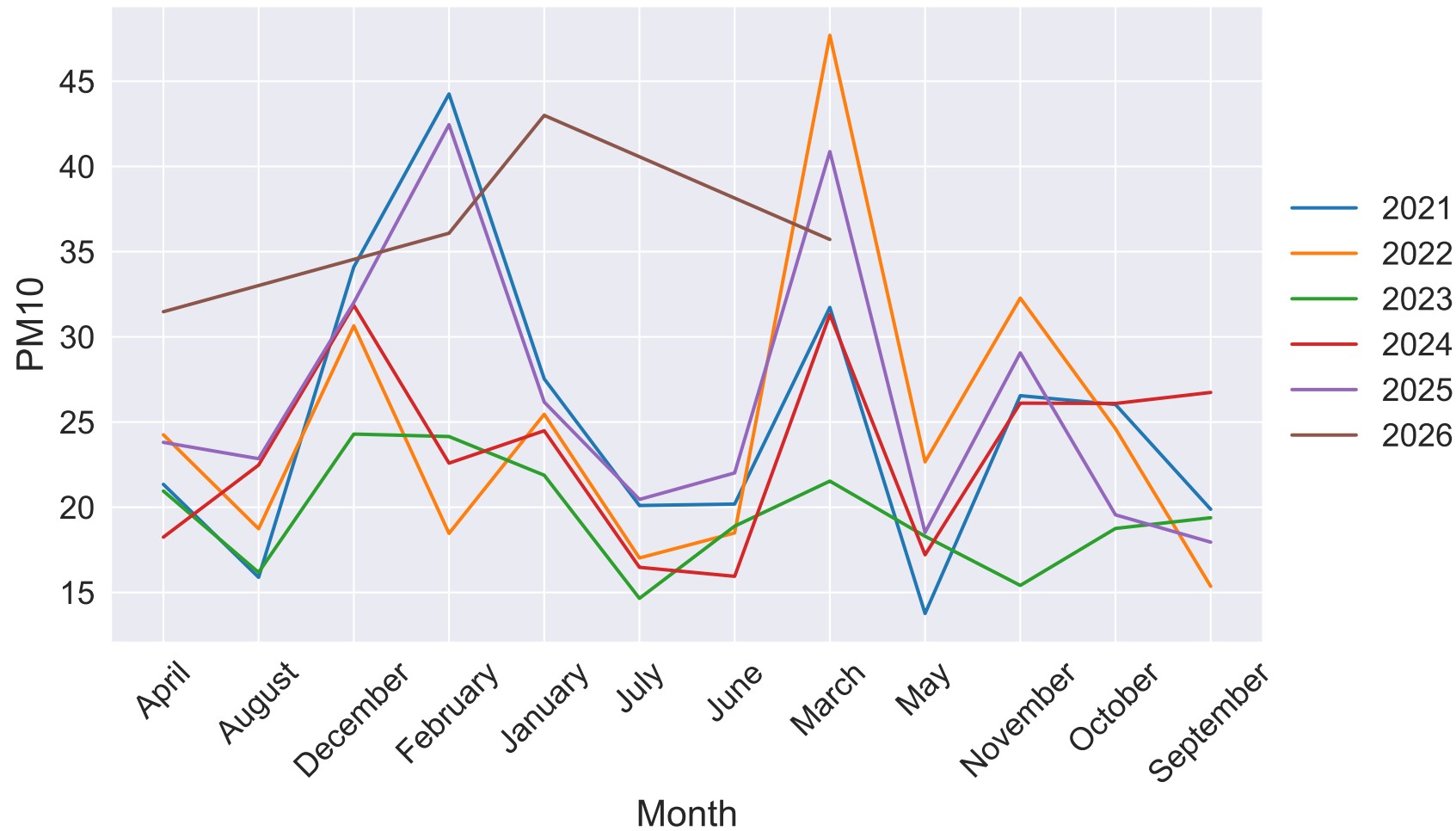
Seasonal Plot - PM10
