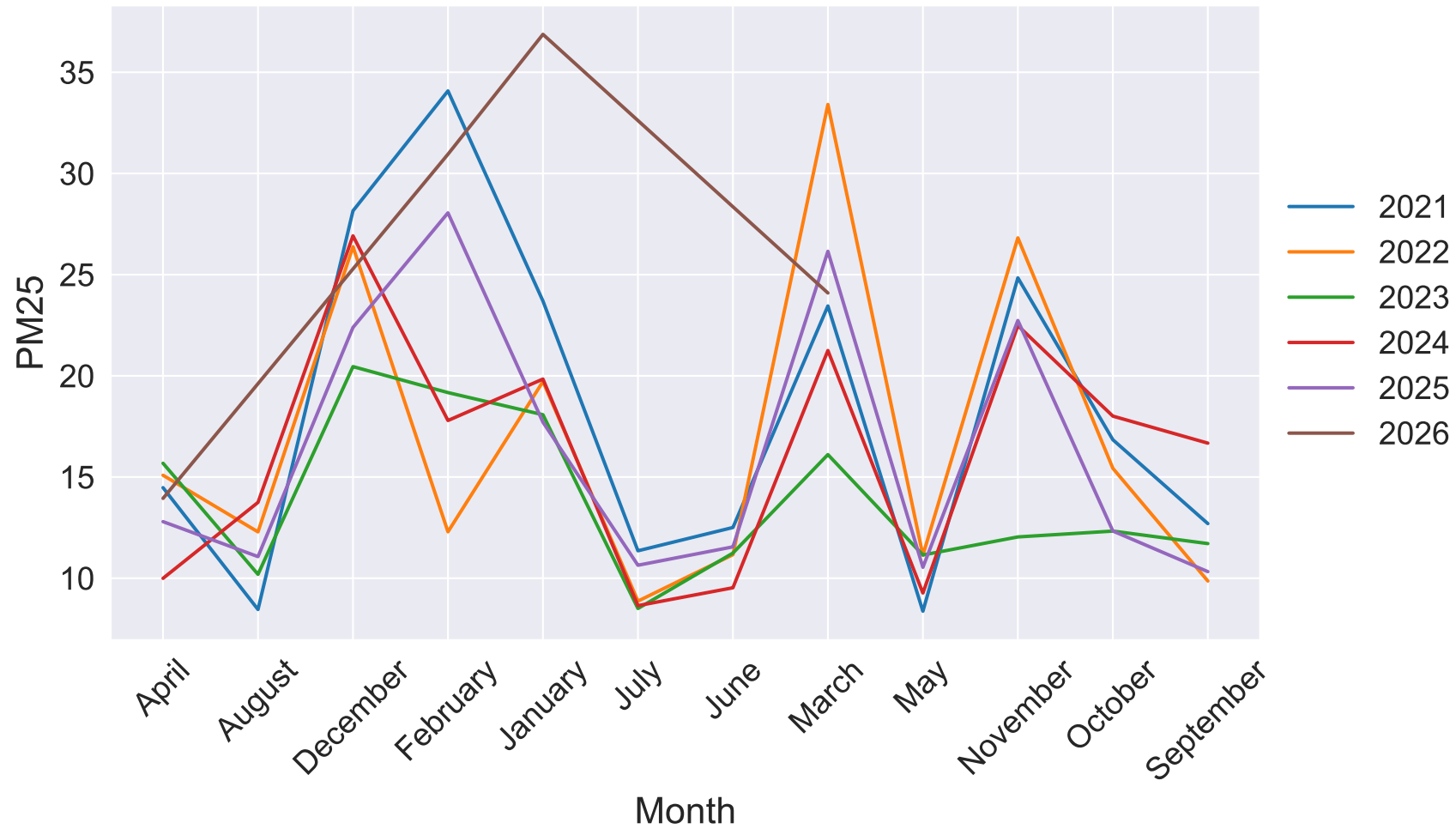
Seasonal Plot - PM25
