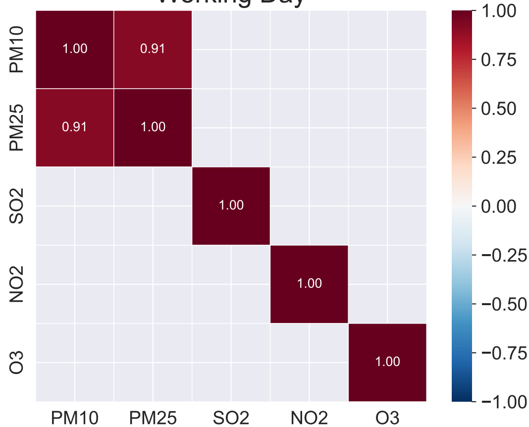
Spearman correlation of pollutants by working day and weekend where |r_s| \geq 0.9
