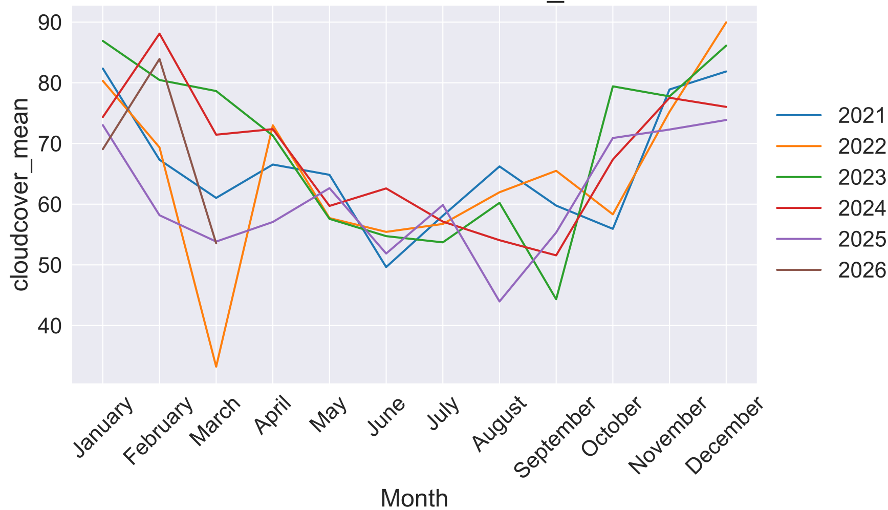
Seasonal Plot - cloudcover_mean
