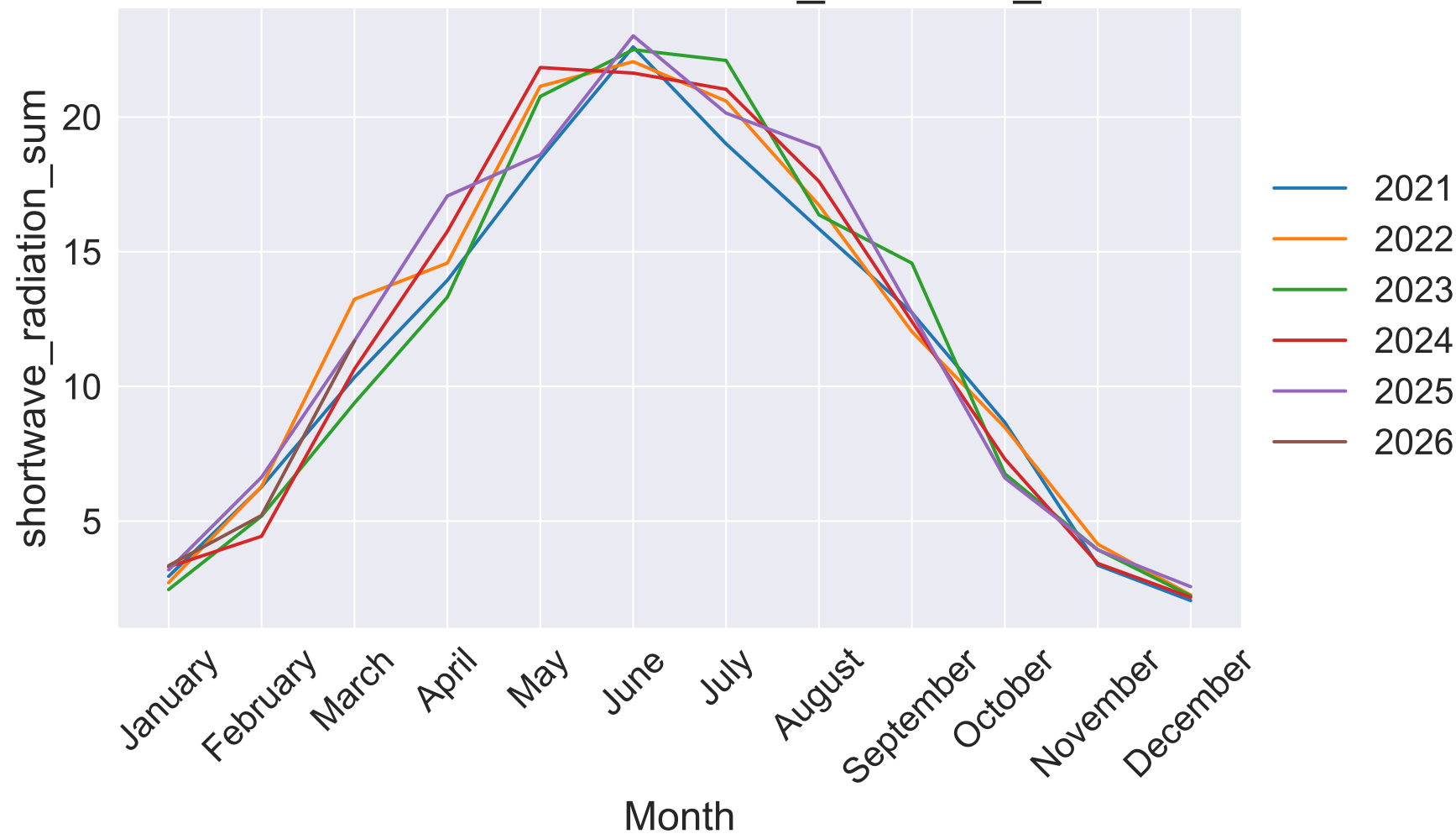
Seasonal Plot - shortwave_radiation_sum
