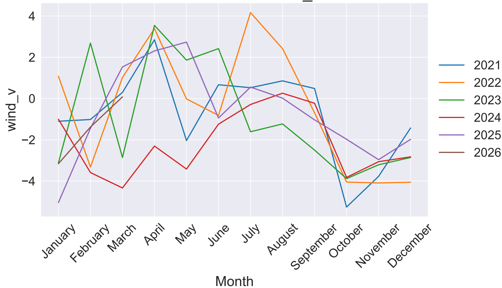
Seasonal Plot - wind_v
