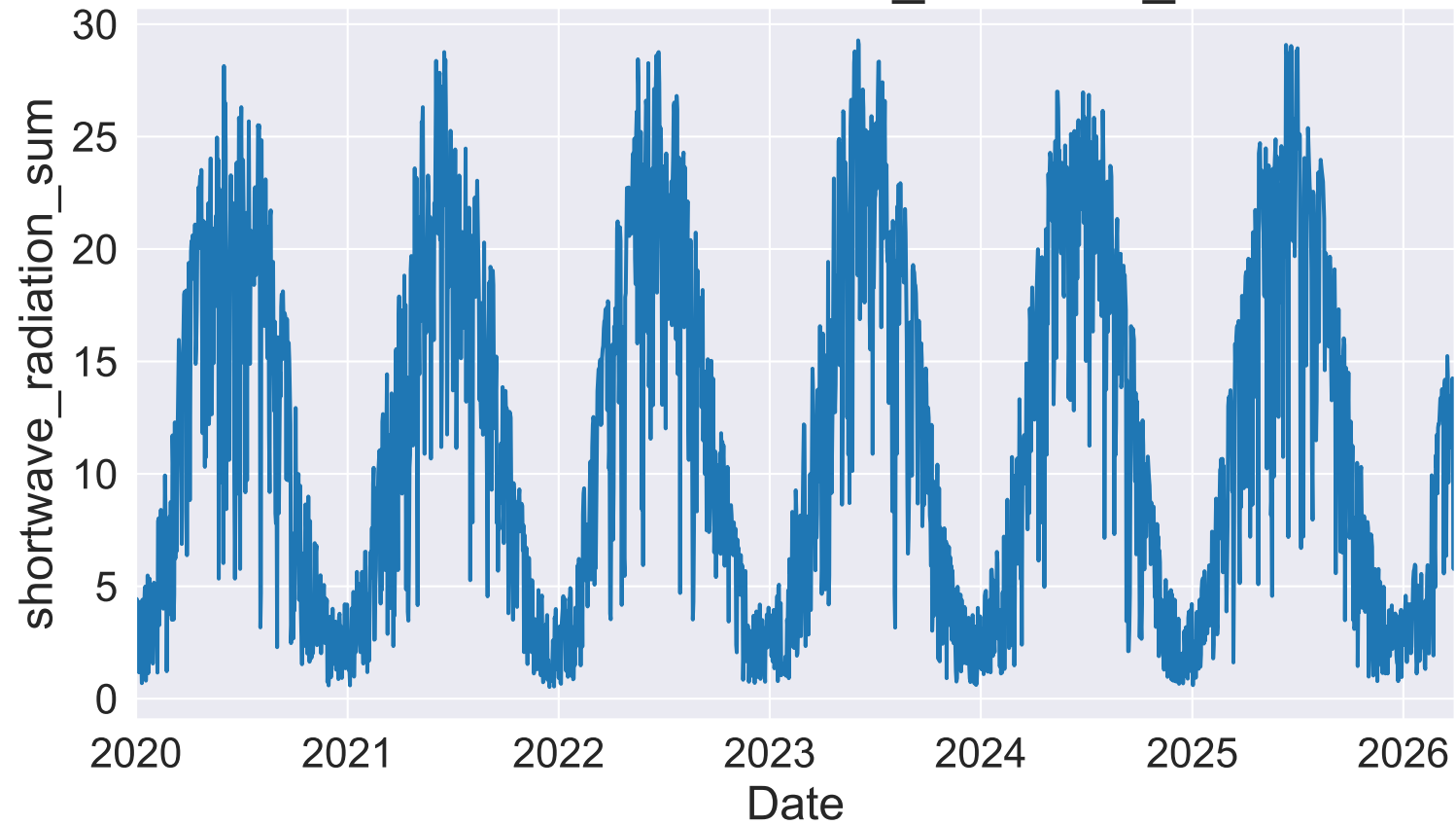
Time series: shortwave_radiation_sum
