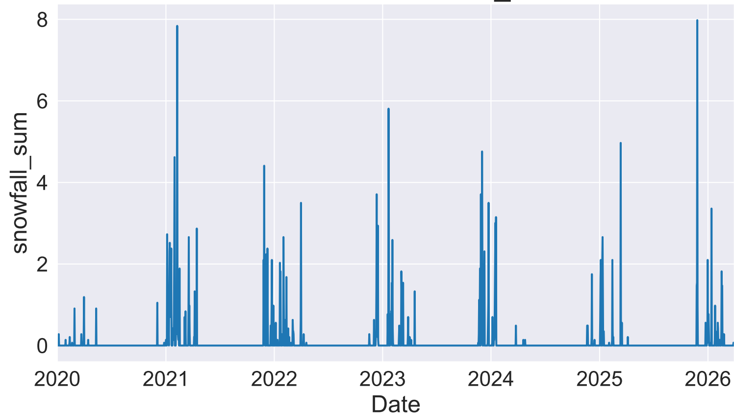
Time series: snowfall_sum
