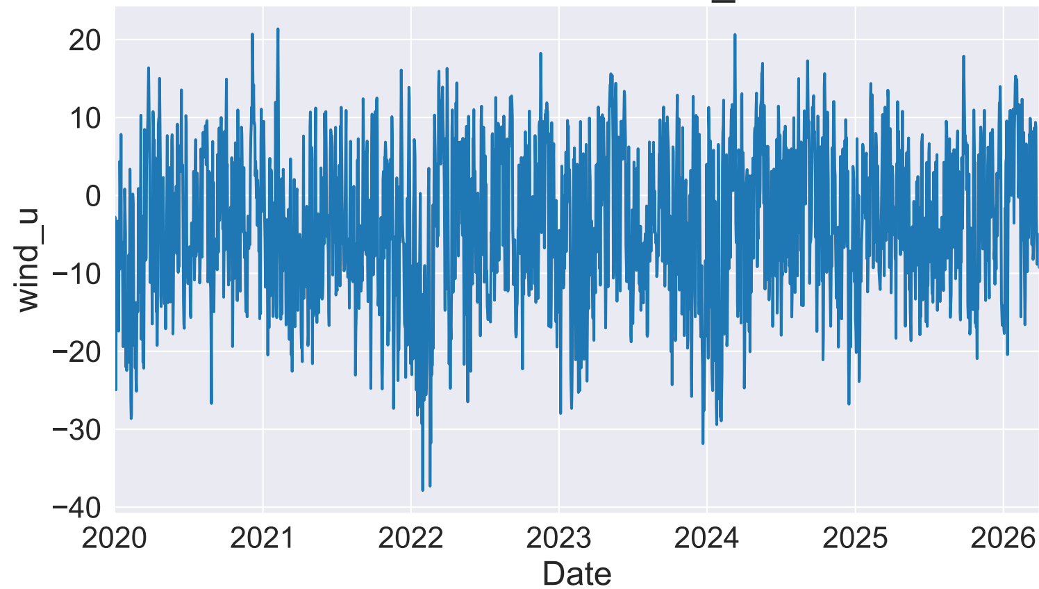
Time series: wind_u
