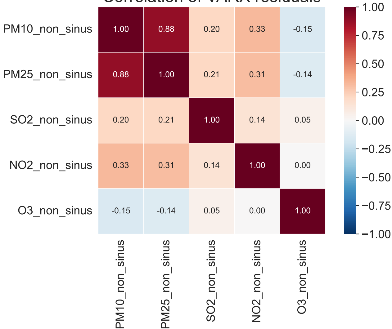
Correlation of VARX residuals
