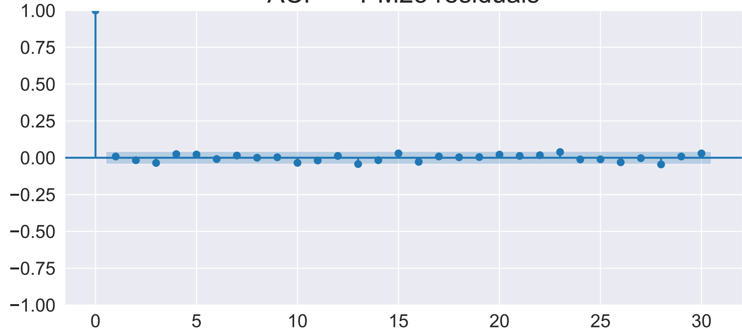
ACF — PM25 residuals
