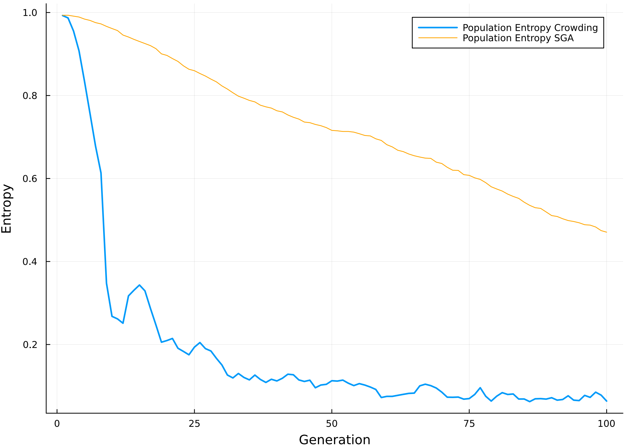
Population Entropy Over Generations
