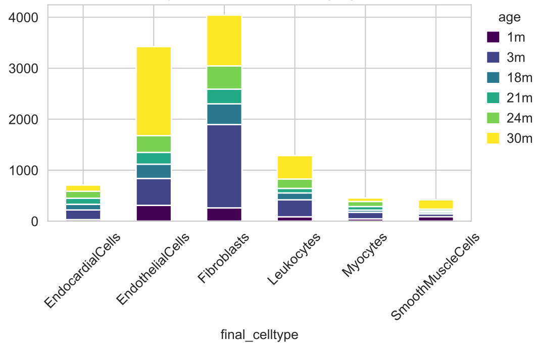
Cell type composition per age group
